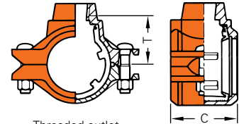
Threaded outlet
